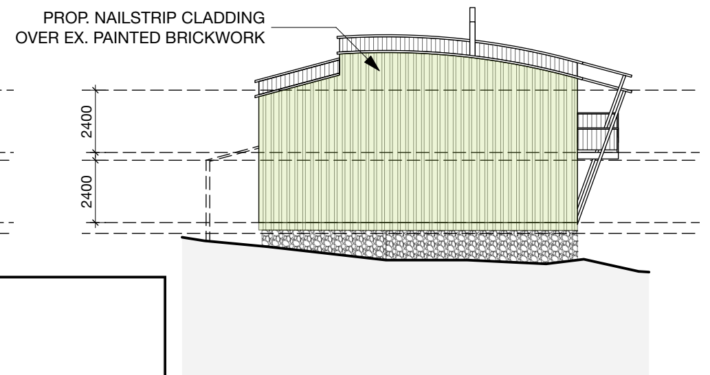
NORTH ELEVATION
