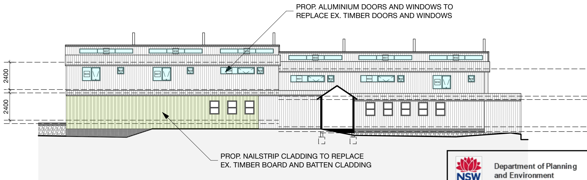
EAST ELEVATION
